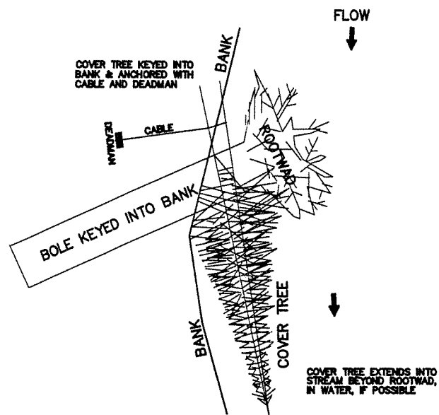
PLAN VIEW TYPICAL
