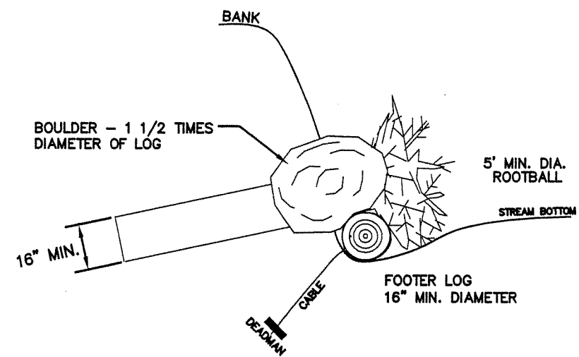
CROSS SECTION TYPICAL
