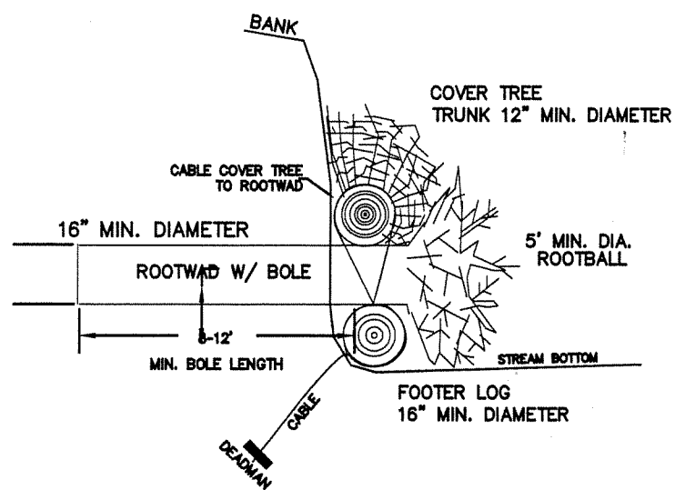
CROSS SECTION TYPICAL
